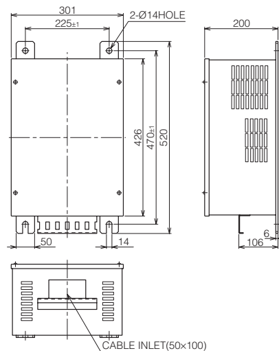
DUAL AC ADAPTER (MKS 066) MASS: 20 kg
